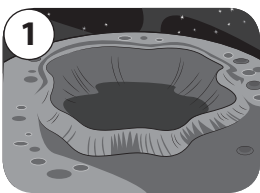
crater
