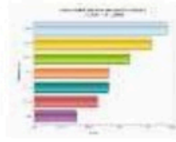
column chart
