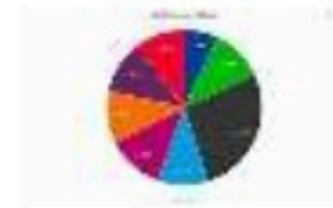
pie chart
